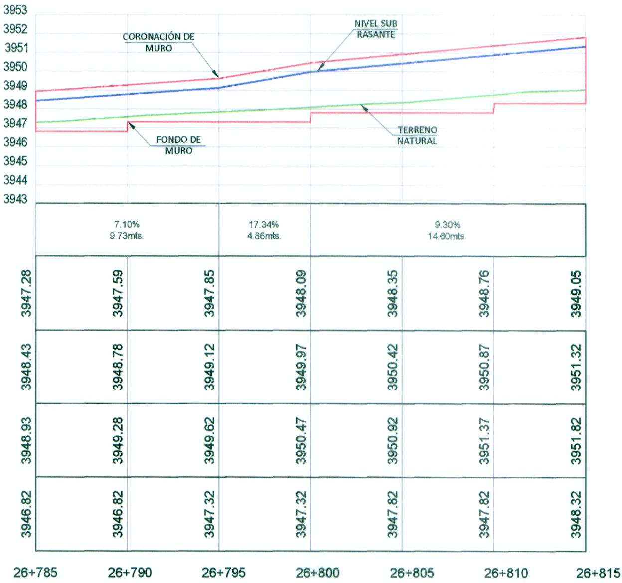
Muro 26+785 - 26+815
