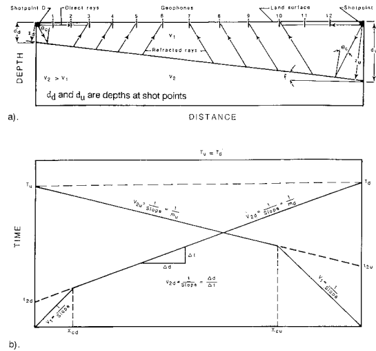
FIG. 6 (a) Seismic Raypaths and (b) Time-Distance Plot for a Two-Layer Model With A Dipping Boundary (9)
