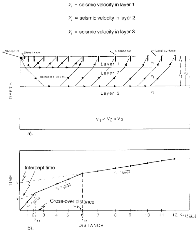
FIG. 5 (a) Seismic Raypaths and (b) Time-Distance Plot for a Three-Layer Model With Parallel Boundaries (9)
