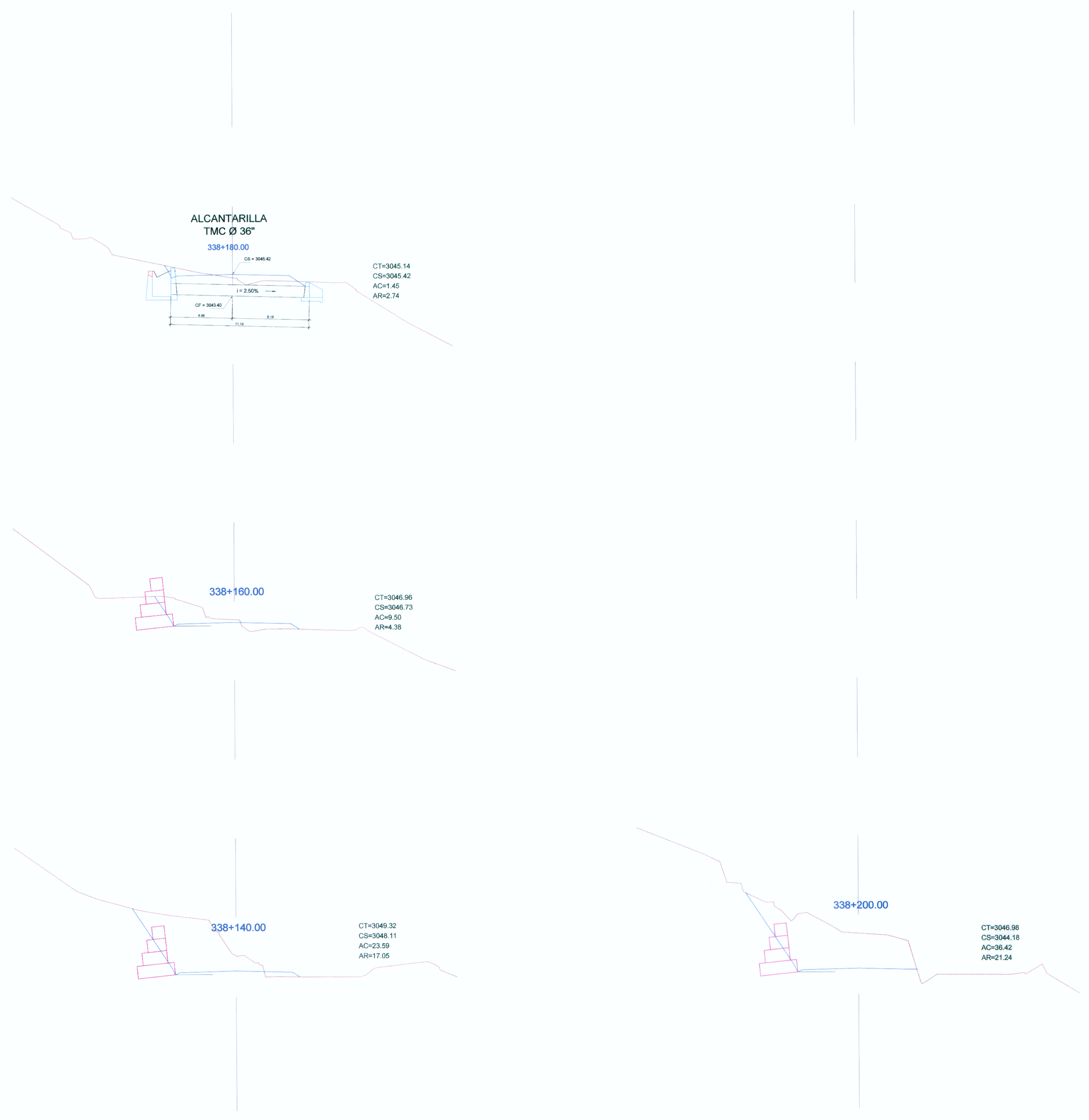
7 GAVION KM. 338+140.00 - KM. 338+200.00
