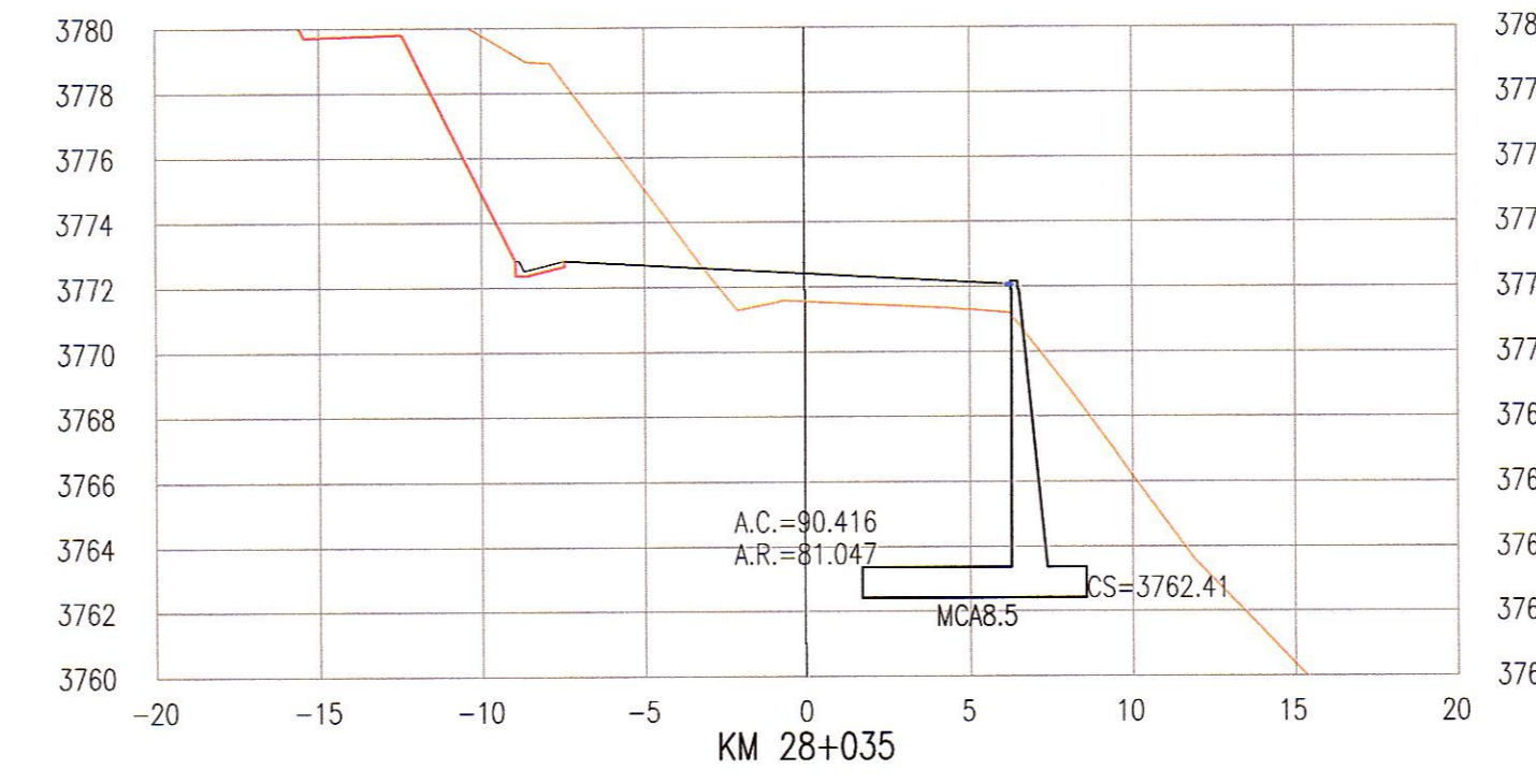
KM 28+012.5 A KM 28+047.5
