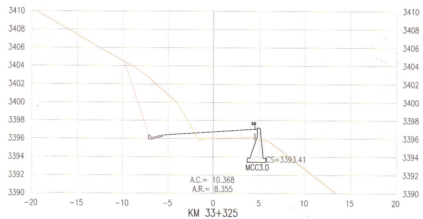
KM 33+322.5 A KM 33+357.5
